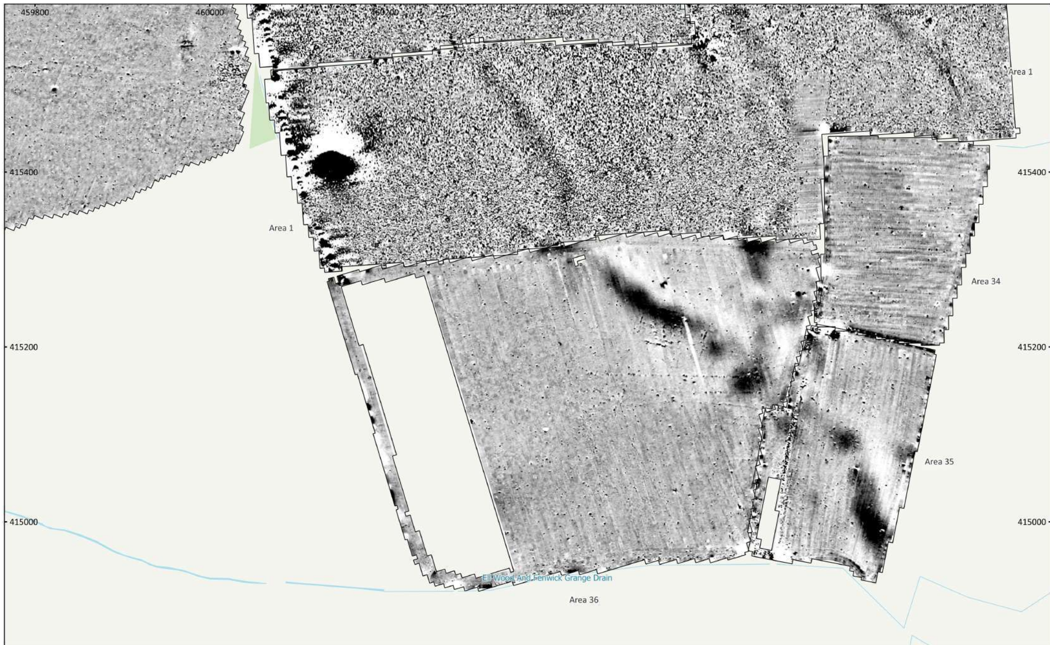
MSSE1569 - Fenwick Solar Farm Scheme, Doncaster Figure 18 - Magnetic Total Field (Lower Sensor) (South (Central)) 1:3,000 @ A3 Copyright Magnitude Surveys Ltd 2023 Contains Ordnance Survey data © Crown Copyright and database right 2023
