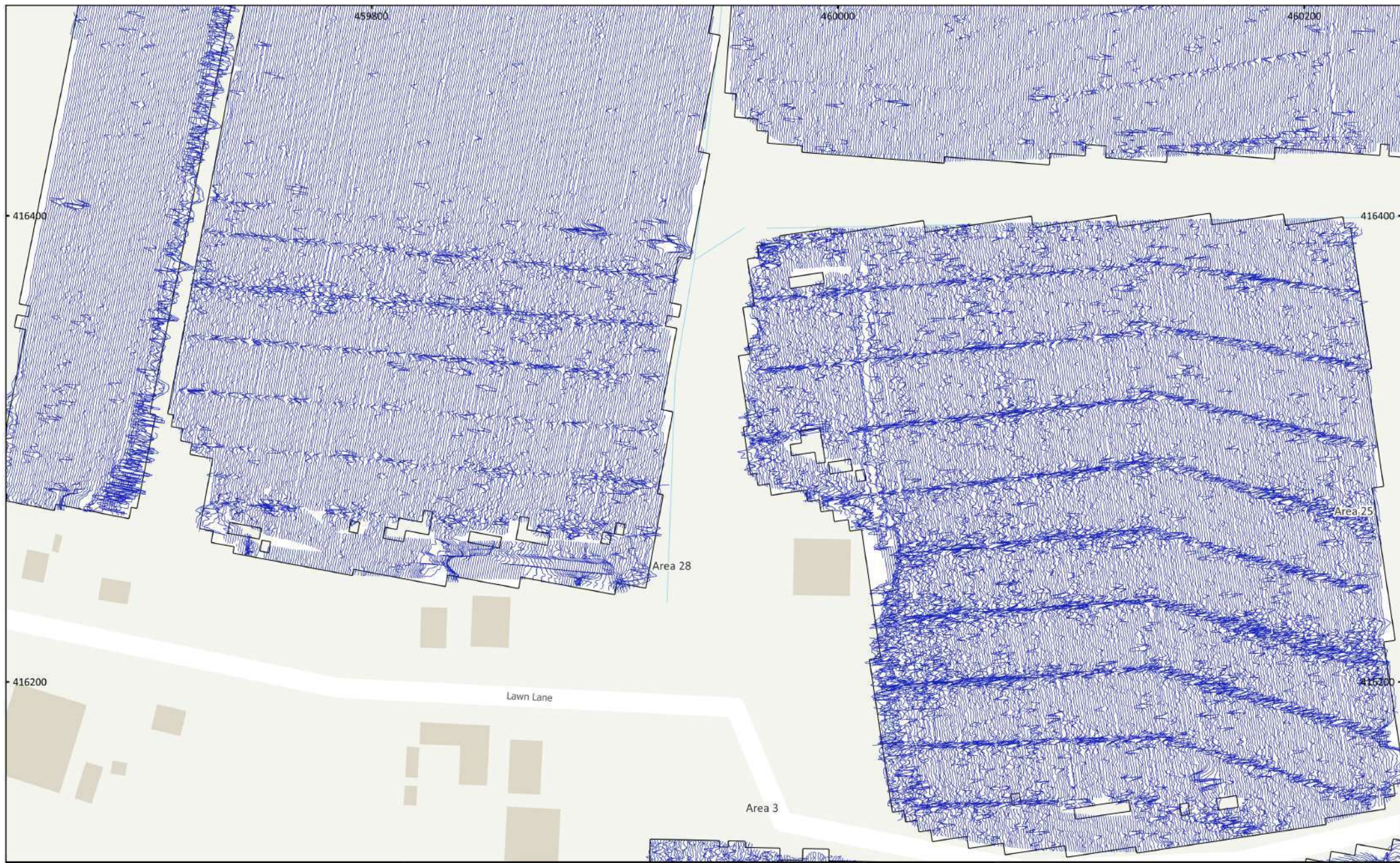
MSSE1569 - Fenwick Solar Farm Scheme, Doncaster Figure 35 - XY Trace Plot (Areas 3, 25, 28 & 32) 30nT/cm at 1:1,500 @ A3 Copyright Magnitude Surveys Ltd 2023 Contains Ordnance Survey data © Crown Copyright and database right 2023
