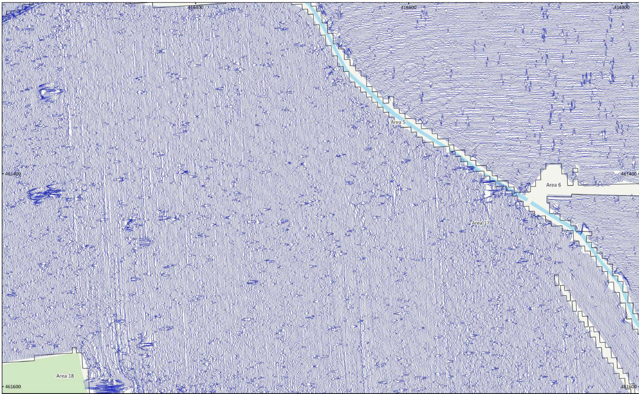
MSSE1569 - Fenwick Solar Farm Scheme, Doncaster Figure 77 - XY Trace Plot (Areas 5, 6, 17 & 18) 30nT/cm at 1:1,500 @ A3 Copyright Magnitude Surveys Ltd 2023 Contains Ordnance Survey data © Crown Copyright and database right 2023
